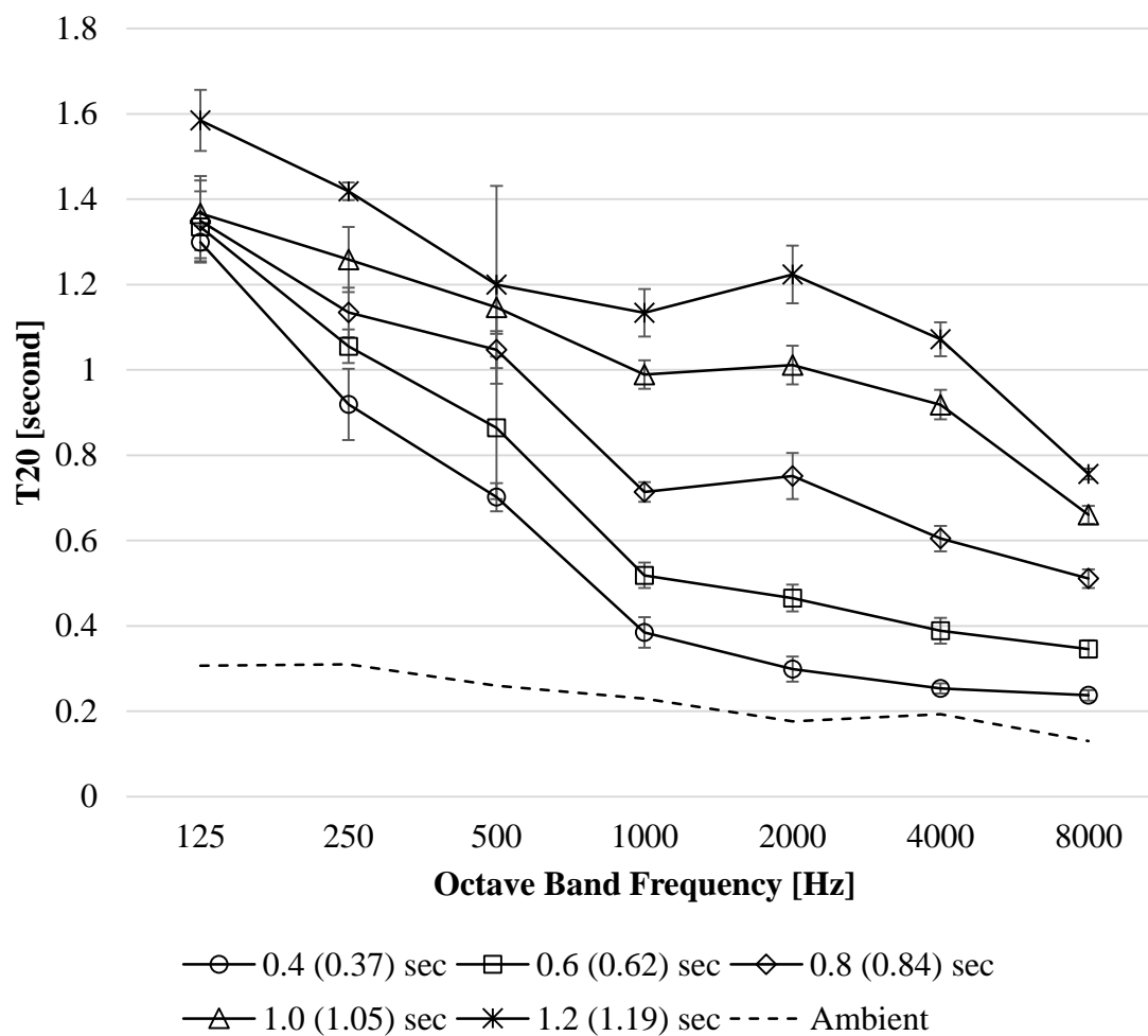
Figure 3.2 - RT in T 20 from 125 Hz to 8000 Hz, measured at the listener position in listening chamber, for the ambient and five RT scenarios from 0.4 to 1.2 seconds. Error bar indicates one standard deviation from 10 in situ measurements. Single numbered T 20 in parenthesis are actual measured RT averaged from 500 Hz to 2000 Hz.
