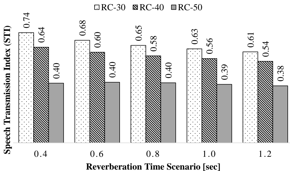
Figure 3.4 - Speech transmission index (STI) for each acoustic condition
